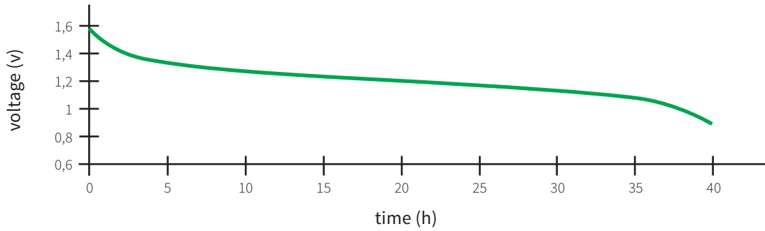
LR20, 3.9 ohms (1h/d) intermittent discharge curve
