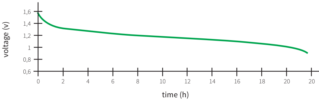
LR20, 2.2 ohms (1h/d) intermittent discharge curve
