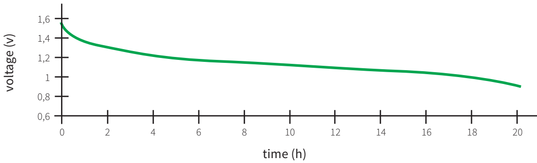
LR20, 2.2 ohms (4m/h, 8h/d) intermittent discharge curve
