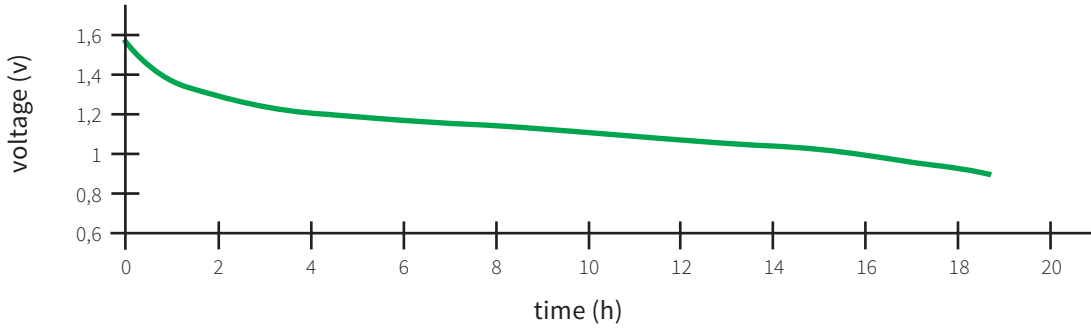
LR20, 2.2 ohms continuous discharge curve
