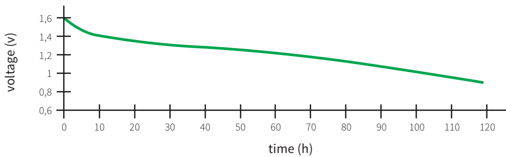
LR20, 10 ohms (4h/d) intermittent discharge curve
